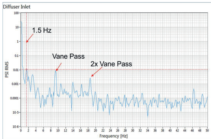
Figure 7: Relevant impeller frequencies from Simcenter STAR-CCM+ at impeller and diffuser inlets.
